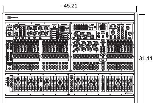
VENUE Profile dimensions
