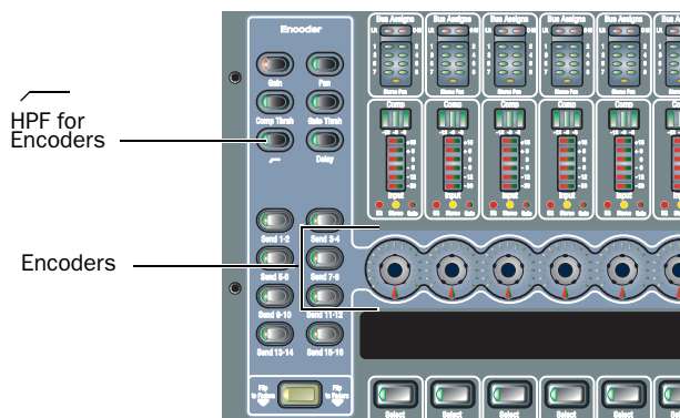
HPF controls for input channels
