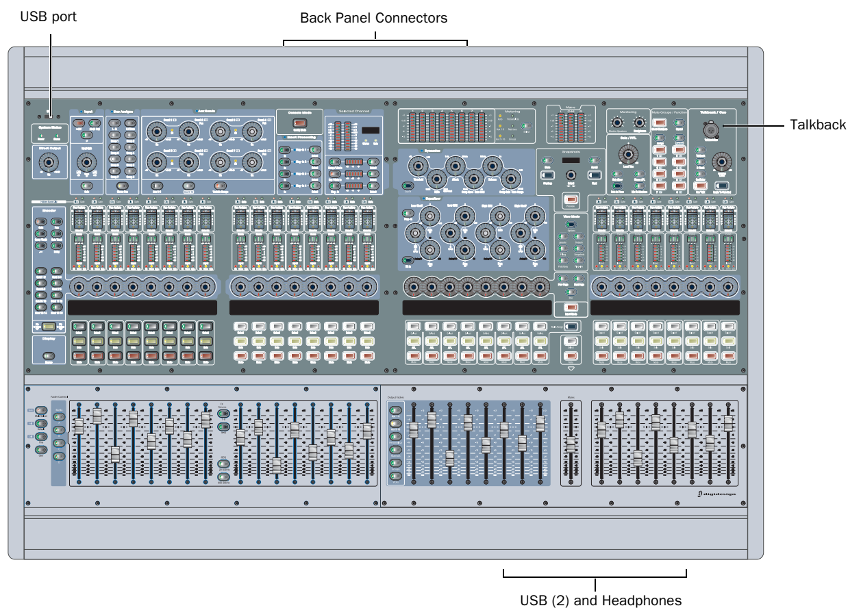
Figure 20. VENUE Profile connectors
