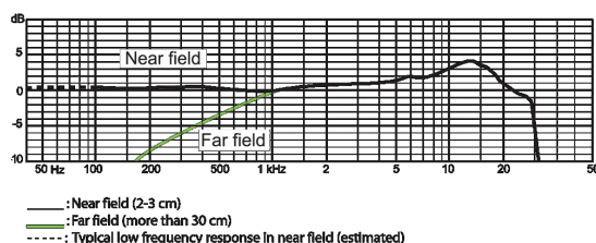
Frequency response of the DPA 4088
