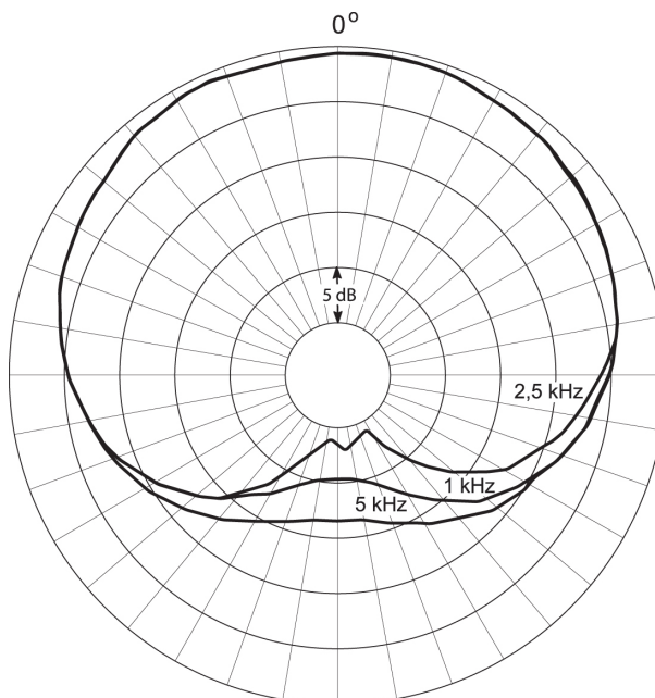
Directional Characteristics of DPA 4088
